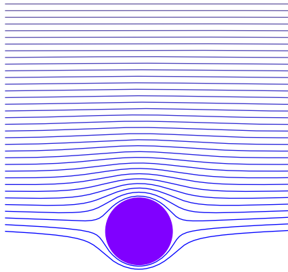
(A) Cas \alpha = 0.1 .
